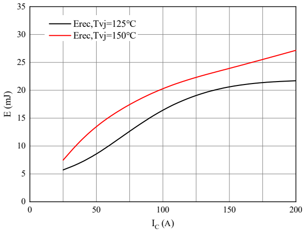
图 7. 开关损耗 二极管 Figure 7. Switching losses of Diode RGon=1Ω, VCE=900V
